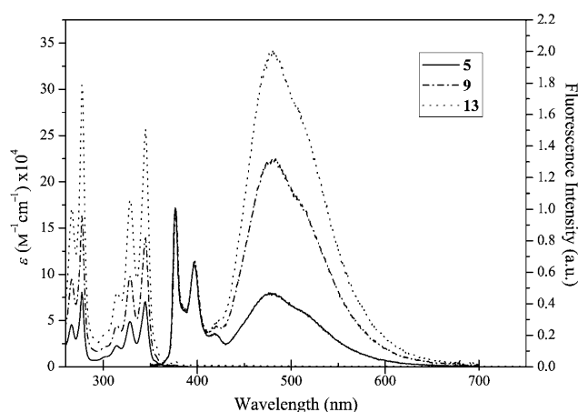
Figure 2. UV absorption and fluorescence ( \lambda_{\text{exc}}=345 nm) spectra of 5 , 9 , and 13 in DMF. The emission profiles were normalized at 377 nm.
