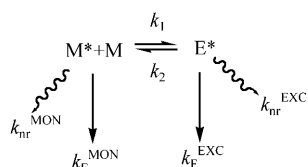
Figure 5. Schematic processes for excimer formation/deactivation. E = excimer, M = monomer, k_{\text{nr}} = non-radiative rate constant.
