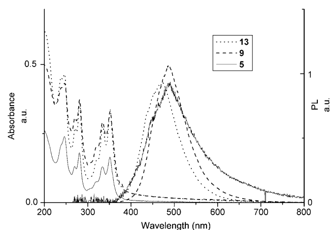
Figure 7. Solid-state (cast-film) absorption and fluorescence spectra of 5 , 9 , and 13 .
