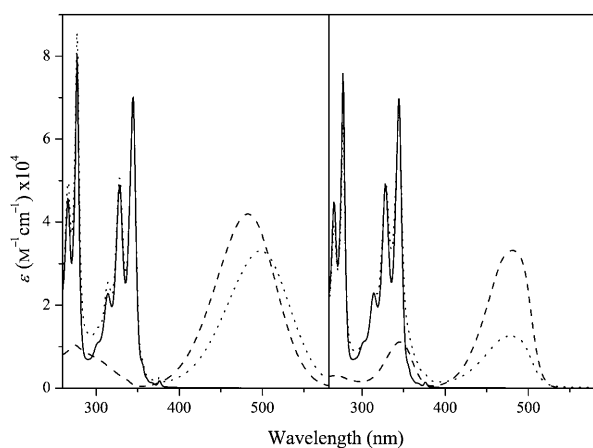
Figure 3. The absorption spectra (dotted line) of 18 (right) in \text{CH}_2\text{Cl}_2 and 20 (left) in DMF were compared to their correspondent donor (solid line) and acceptor (dashed line) moieties.
