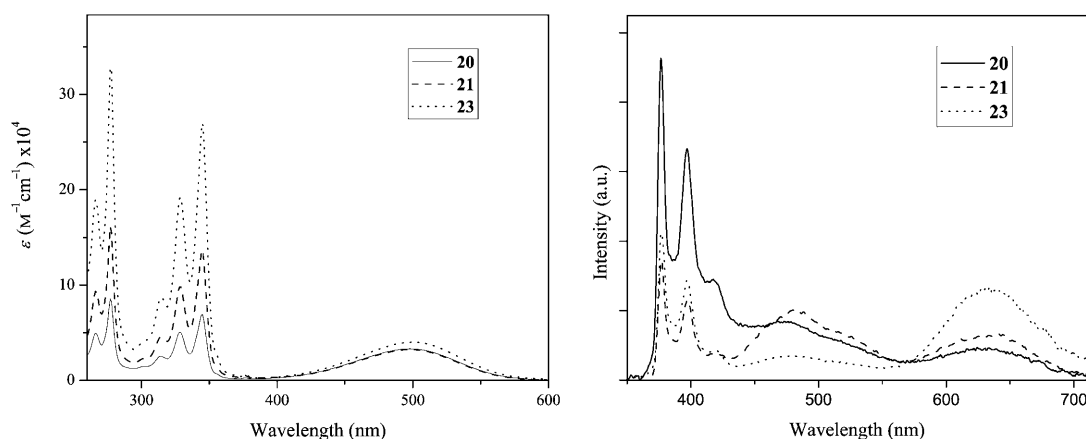
Figure 6. Absorption spectra (left) and fluorescence spectra (right) of 20–23 . The intensity of the emission profile was divided to the absorbance of the sample at \lambda_{\text{exc}}=345 nm.
