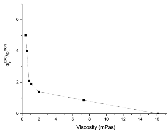
Figure 1. Plot of the \Phi_F^{\text{EXC}}/\Phi_F^{\text{MON}} variation with the viscosity \eta of the solvent. The line is just a guide for the eye.
