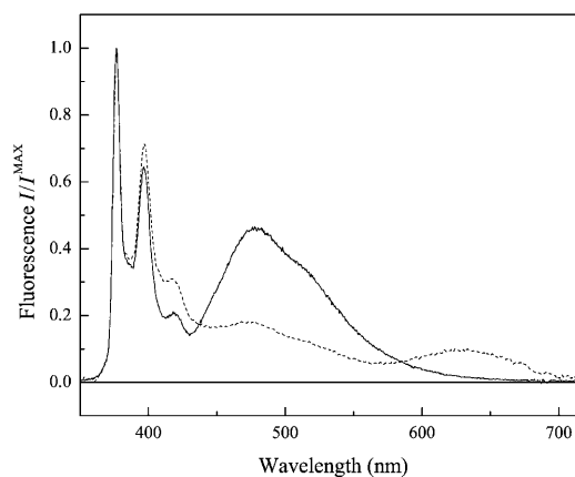
Figure 4. Normalized emission spectra of 20 (dashed line) and 5 (continuous line) in DMF.
